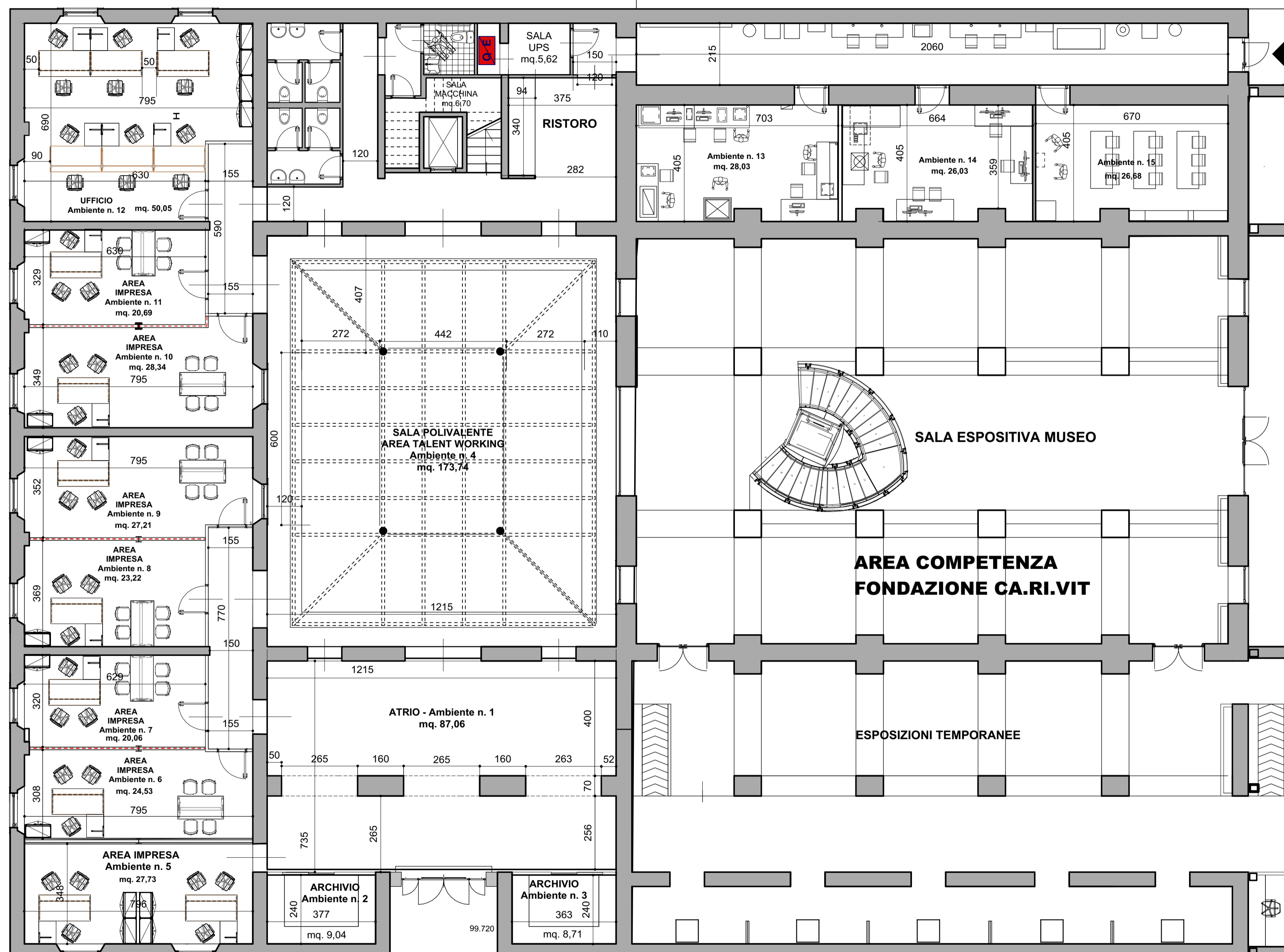
PLANIMETRIA PIANO TERRA
